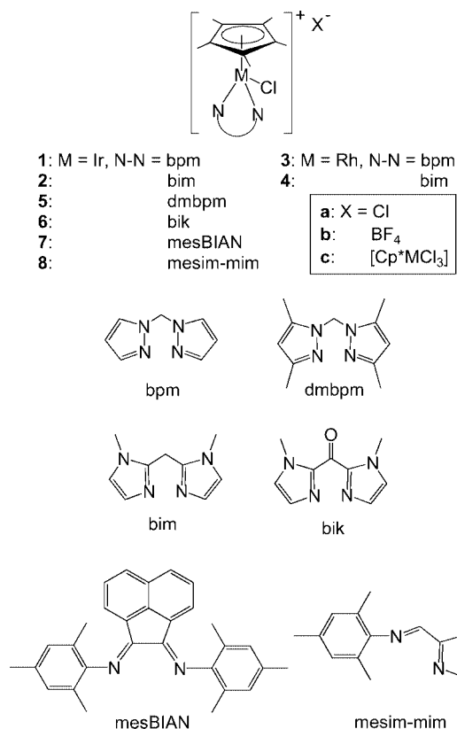
Figure 1. The general structure of complexes 1a–8b and 1a–3c where N–N = bpm = bis(pyrazol-1-yl)methane; bim = bis(1-methylimidazol-2-yl)methane; dmbpm = bis(3,5-dimethylpyrazol-1-yl)methane; bik = bis(1-methylimidazol-2-yl) ketone; mesBIAN = bis(2,4,6-trimethylphenylimino)acenaphthene; mesim-mim = (2,4,6-trimethylphenyl)imino-(1-methylimidazol-2-yl)methane.
