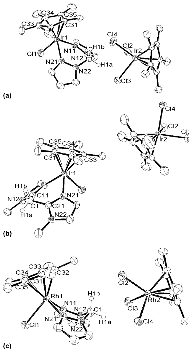
Figure 2. ORTEP depiction of (a) [Cp * IrCl(bpm)][Cp * IrCl 3 ] ( 1c ); (b) [Cp * IrCl(bim)][Cp * IrCl 3 ] ( 2c ); and (c) [Cp * RhCl(bpm)][Cp * RhCl 3 ] ( 3c ) at 50% thermal ellipsoids for the non-hydrogen atoms.
