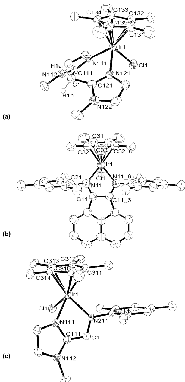
Figure 3. ORTEP depiction of (a) [\text{Cp}^*\text{IrCl}(\text{bim})]^+ ( 2b ); (b) [\text{Cp}^*\text{IrCl}(\text{mesBIAN})]^+ ( 7b ) and (c) [\text{Cp}^*\text{IrCl}(\text{mesim-mim})]^+ ( 8b ) at 50% thermal ellipsoids for the non-hydrogen atoms.
